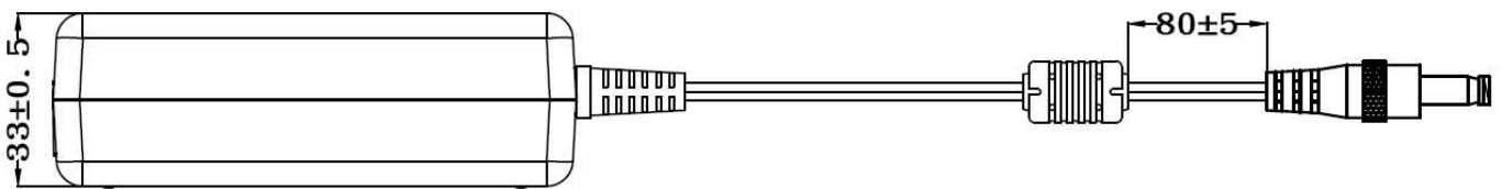
SIDE VIEW
