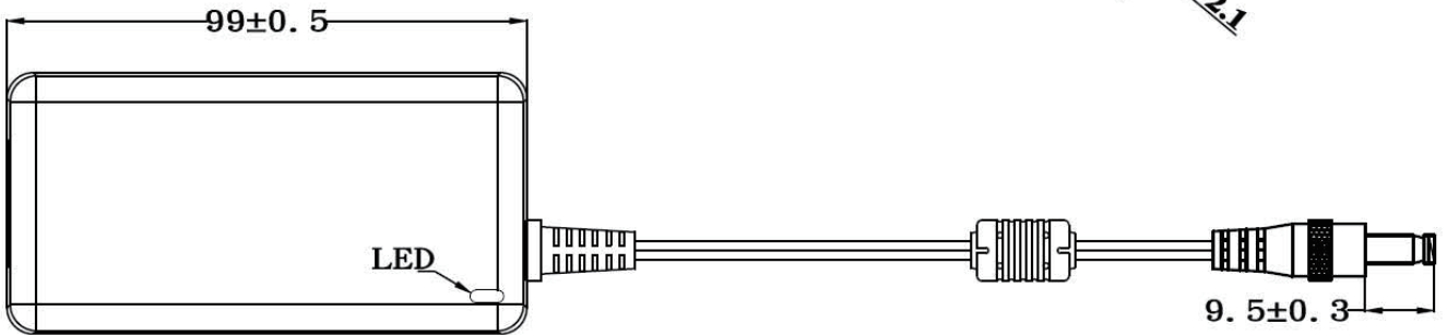
TOP VIEW
